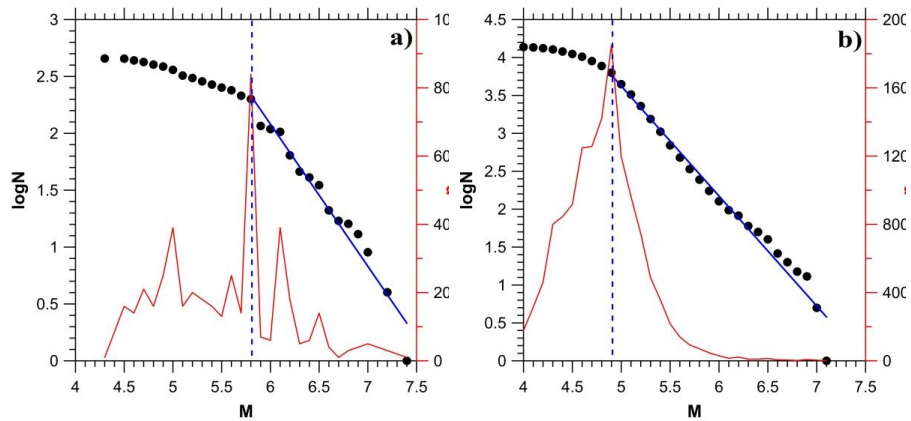
Figure 8 - Gutenberg-Richter distribution of M-AR earthquakes for two time intervals: a) 1920-1963 and b) 1964-2014.
