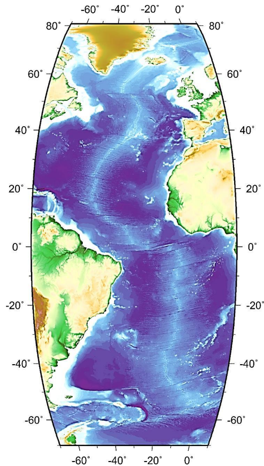
Figure 1 - Map of the Mid-Atlantic Ridge (M-AR).
